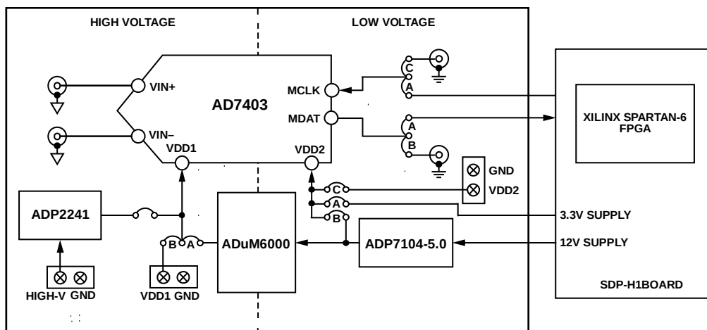
Figure 13. EVAL-AD7403FMCZ Block Diagram
