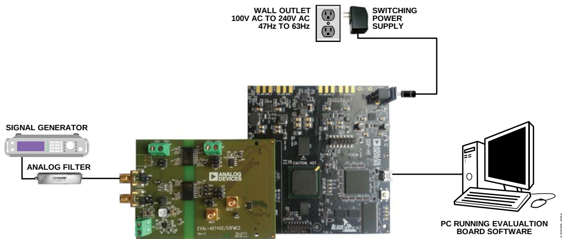
Figure 1. Typical Setup ( EVAL-AD7403FMCZ on Left and EVAL-SDP-CH1Z on Right)
